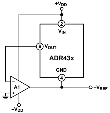
Figure 36. Negative Reference
